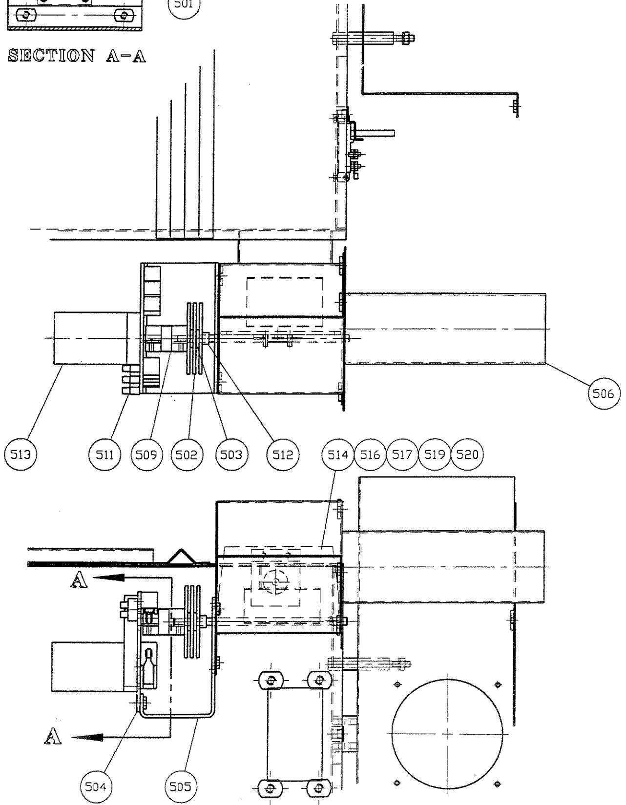
DAMPER CONTROL ASS'Y 0690S20213
